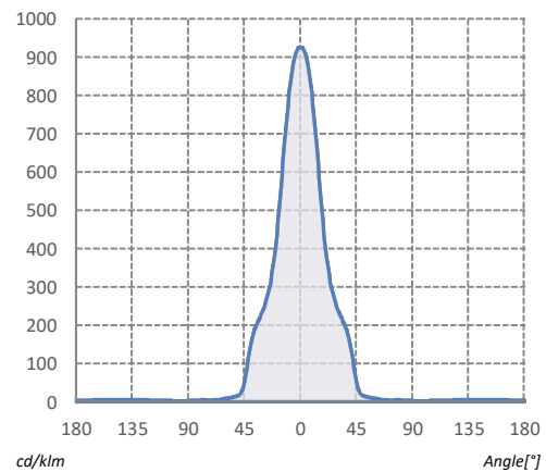
Cartesian diagram
